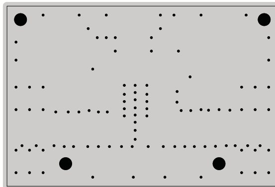
Layer 2: Ground
